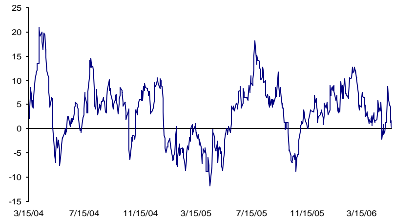
CMI 50-Day Moving Average Spread: Last Two Years
